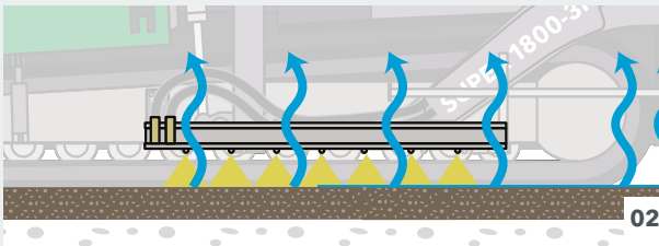
Hot bitumen emulsion at a temperature between 158 to 176 °F (70 to 80 °C) is applied by the spray paver.
