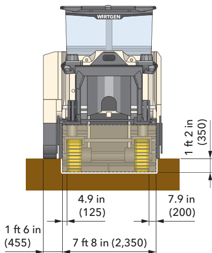
Rear view of cold recycler W 240 CR/W 240 CRi, dimensions in American standard and mm
