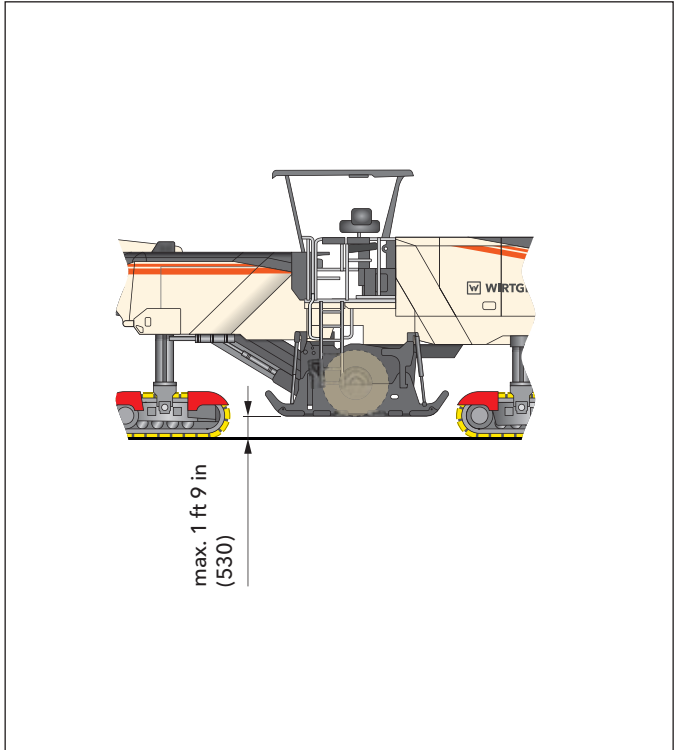
Ground clearance of cold recycler W 380 CR/W 380 CRi, dimensions in American standard and mm
