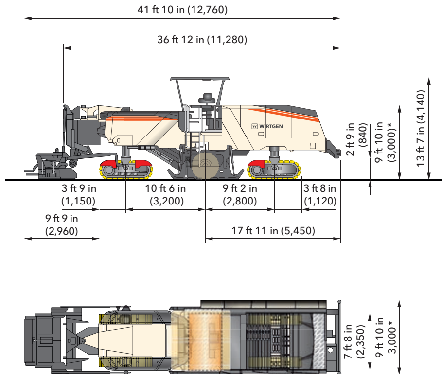
Cold recycler W 240 CR/W 240 CRi including paving screed and spreading auger, dimensions in American standard and mm * = Dimensions for low-loader transport
