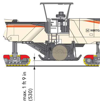
Ground clearance of cold recycler W 240 CR/W 240 CRi, dimensions in American standard and mm
