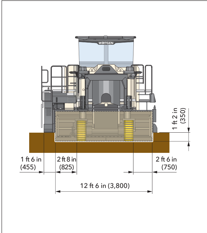
Rear view of cold recycler W 380 CR/W 380 CRi, dimensions in American standard and mm
