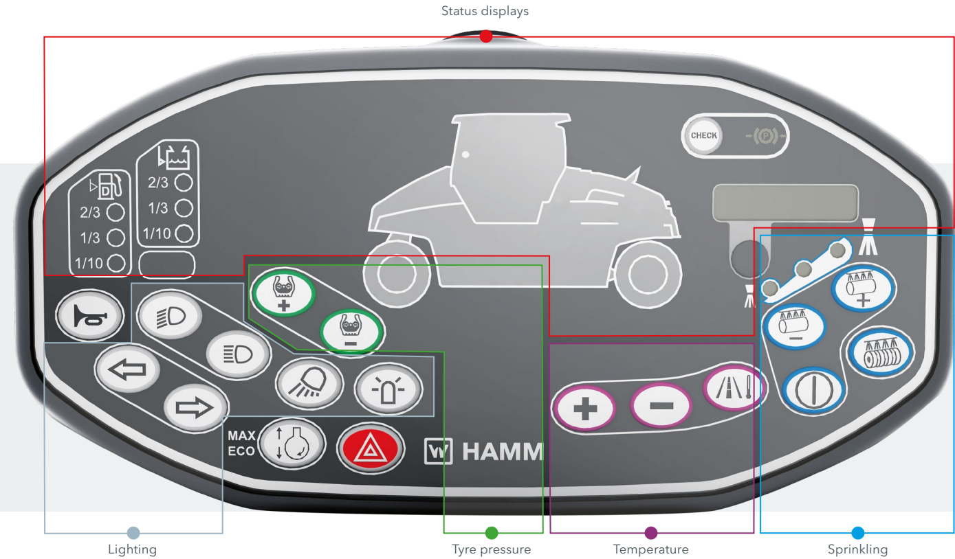
Dashboard on the Tier 3 machines
