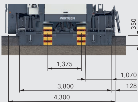
W 220 Fi with 3.8 m milling drum assembly
